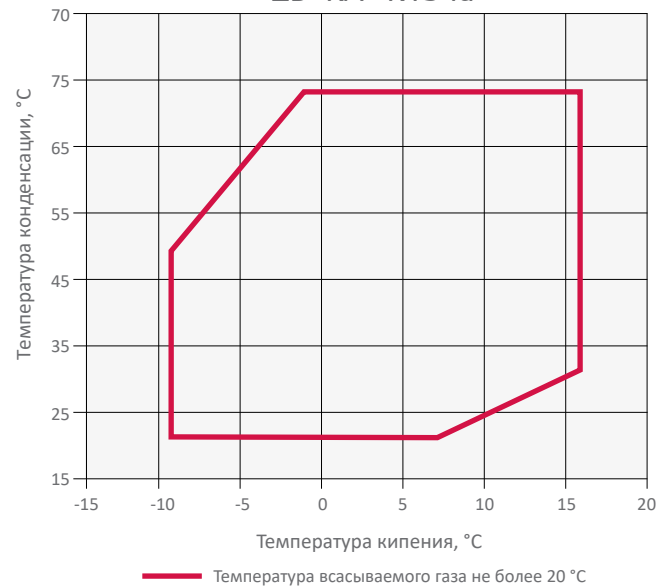
ZB*KA - R134a
