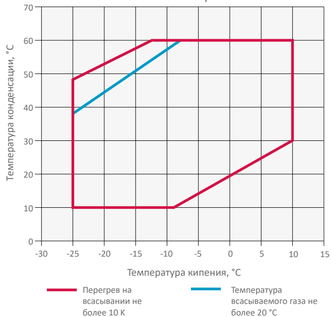
ZF*KA - R448A/R449A
