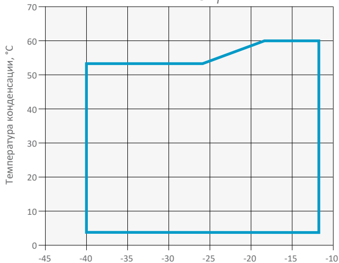
ZF*KA - R448A/R449A
