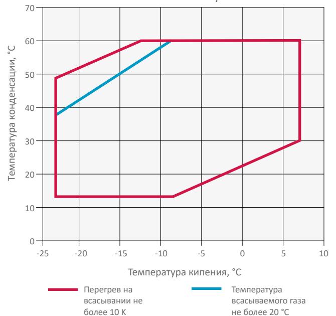
ZB*KA - R448A/R449A
