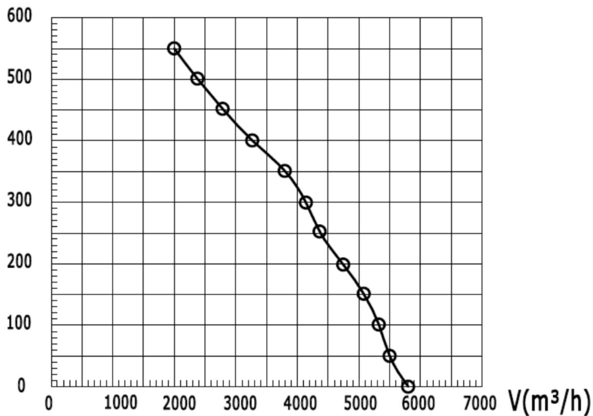
Airflow curves
