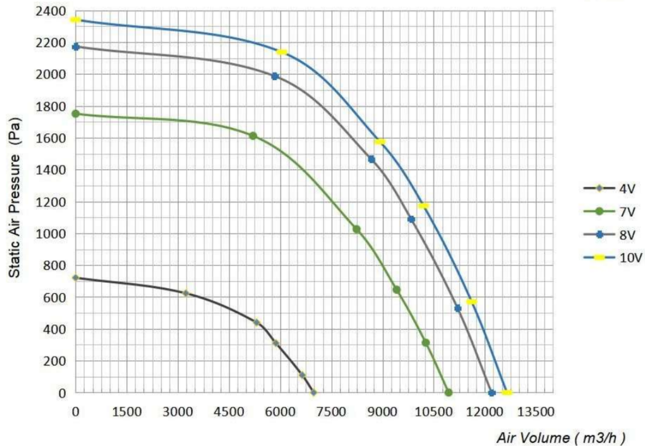
P-Q Curve
