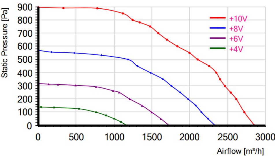
Airflow curve
