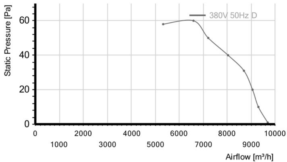
Airflow curve
