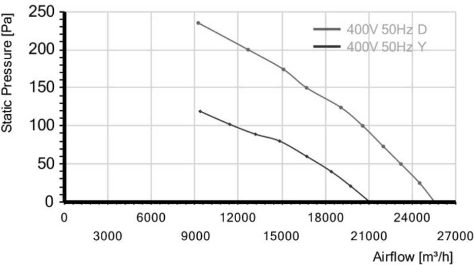
Airflow curve
