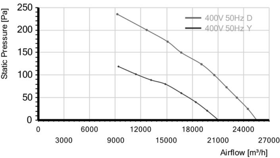
Airflow curve
