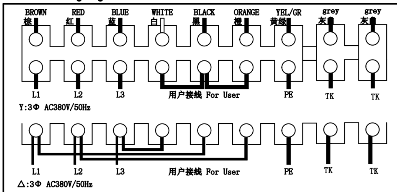
The external wiring diagram:
