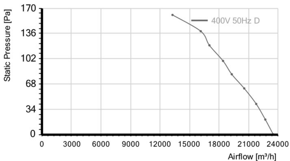
Airflow curve
