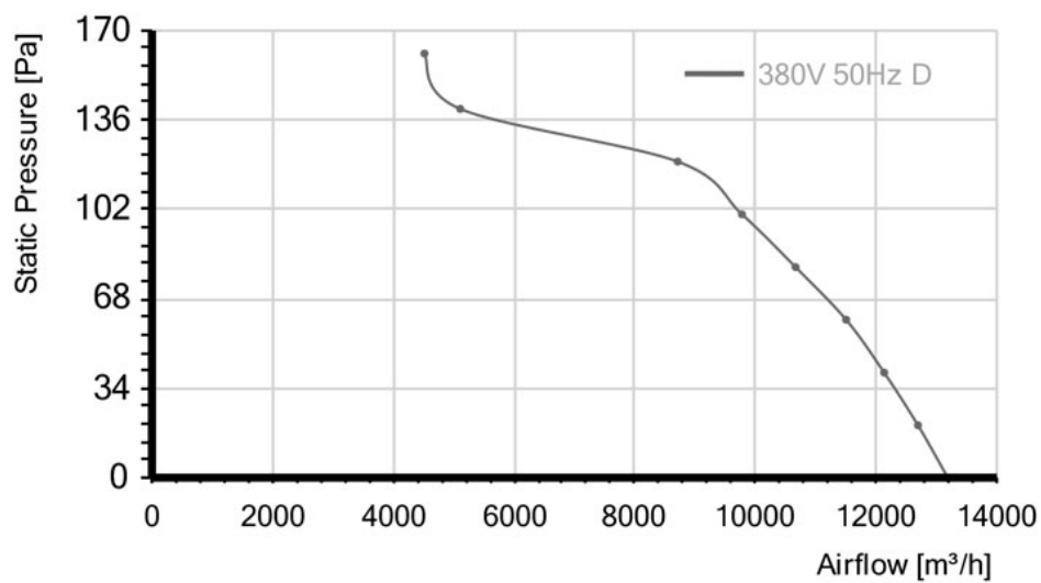
Airflow curve
