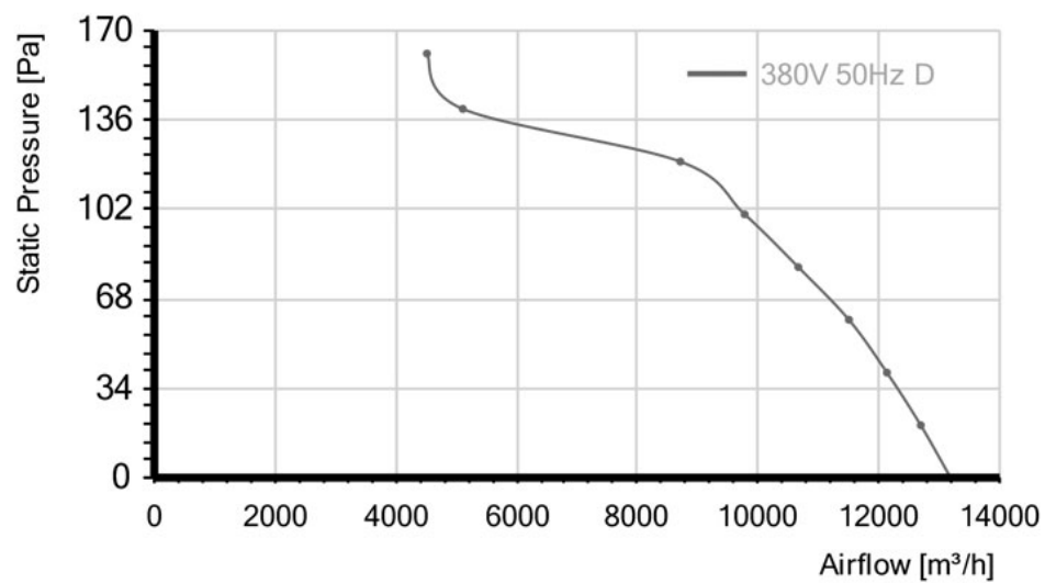
Airflow curve
