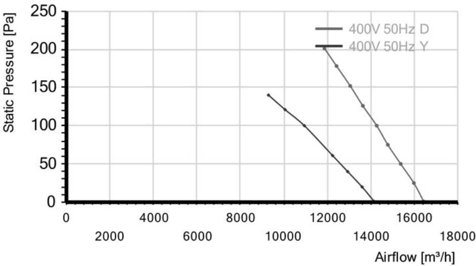
Airflow curve
