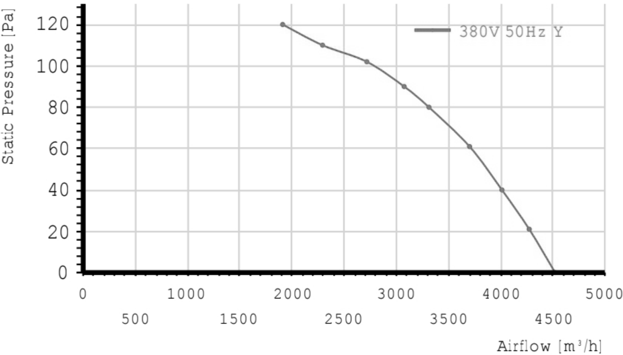
Airflow curve
