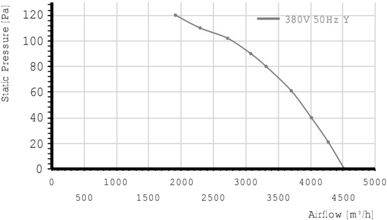
Airflow curve
