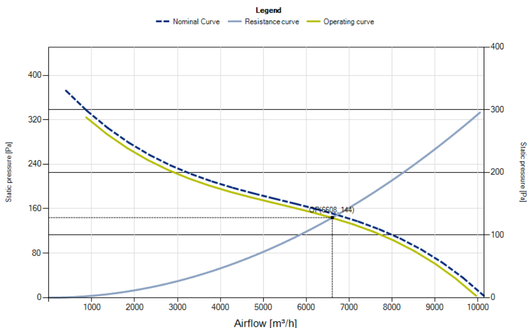
Static pressure
