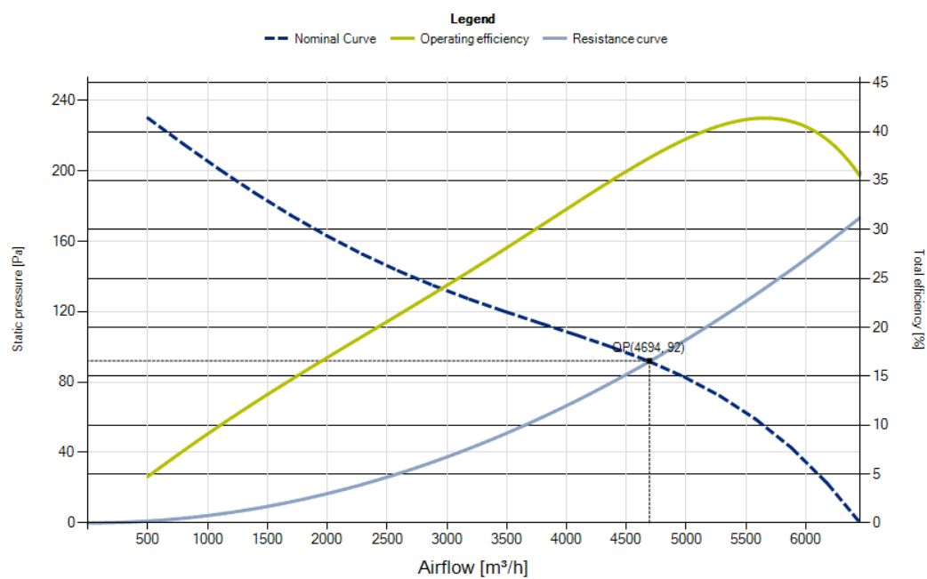
Total efficiency
