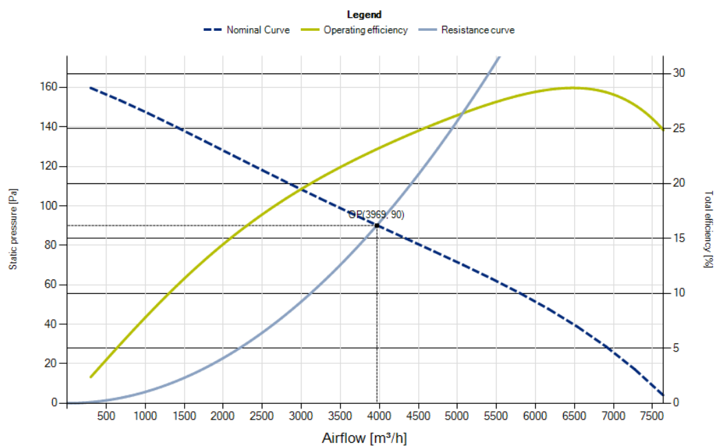
Total efficiency
