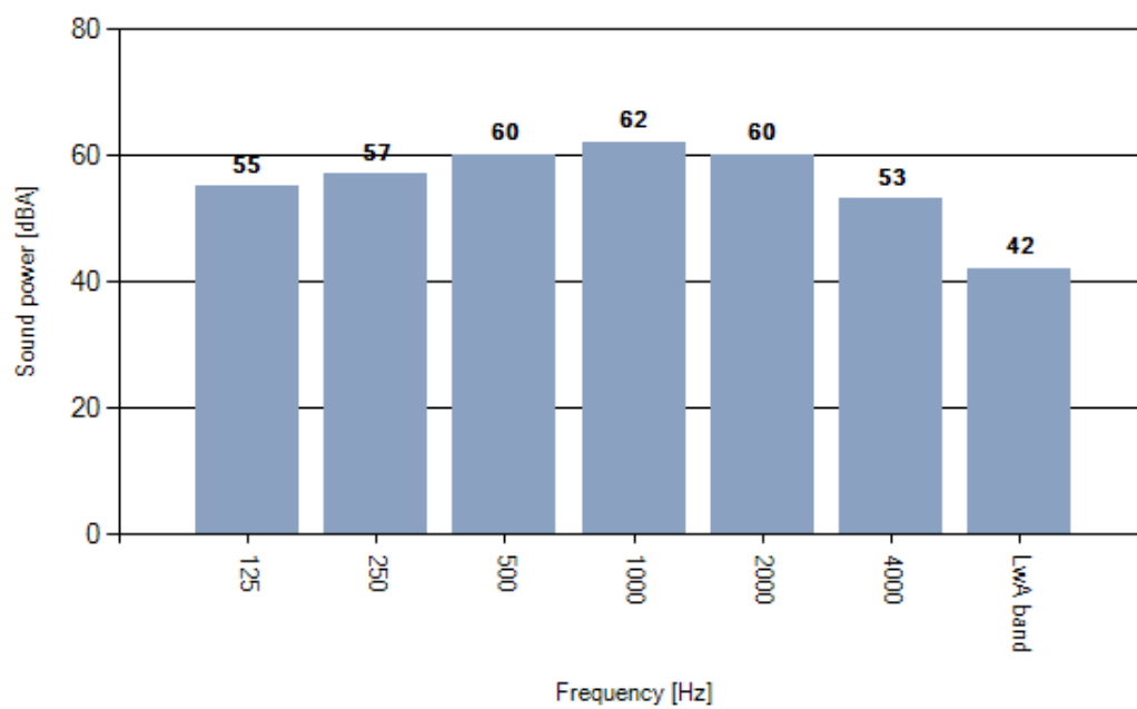
Weighted octave sound power spectrum
