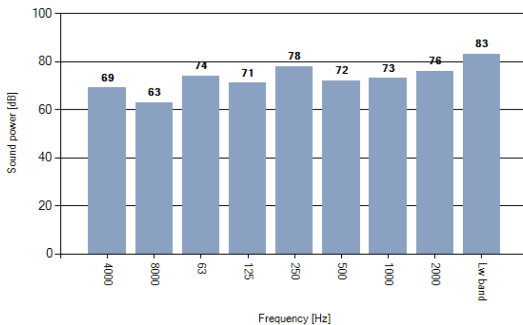
Unweighted octave sound power spectrum
