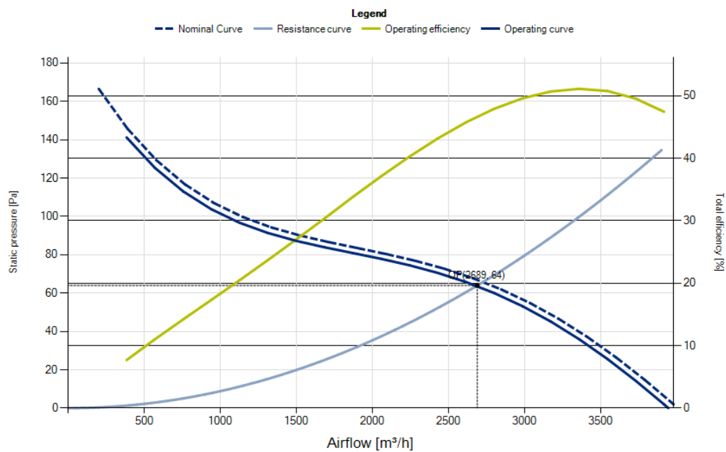
Total efficiency
