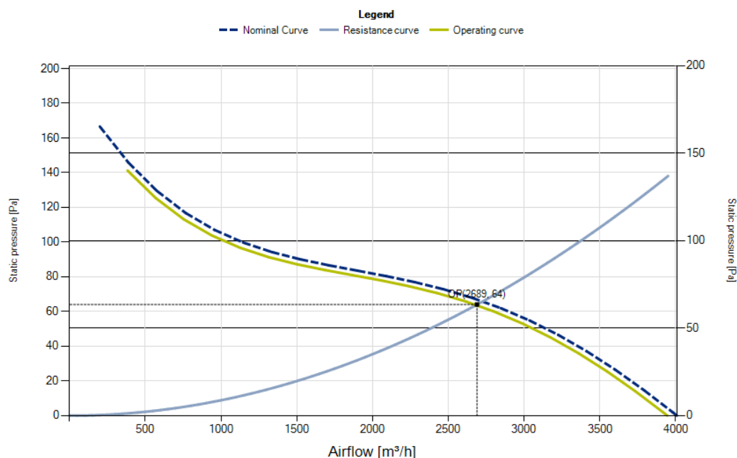
Static pressure
