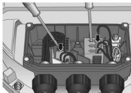
Fig. 3: Connection of cables at terminals
