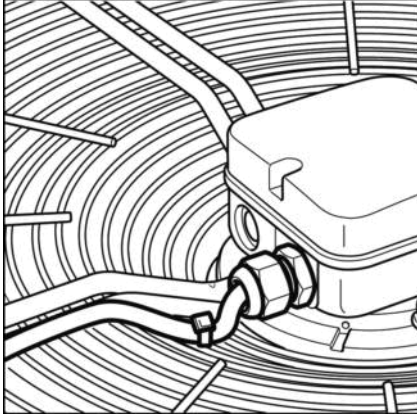
When routing the cable, ensure that the screwed cable glands are arranged at the bottom. The cables must always be routed downwards.
