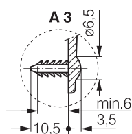
Barbed inserts
