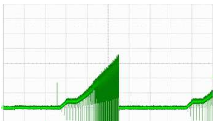
Locked rotor current @ 24 V ( I = 1\text{A/div} ; t = 1\text{s/div} )
