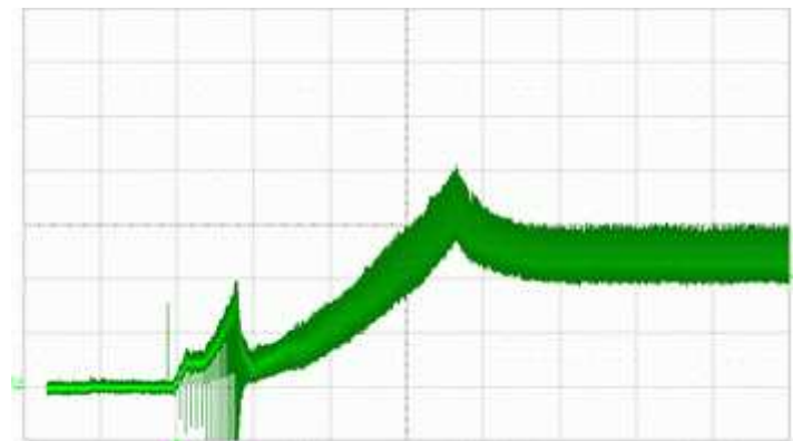
Start-up current @ 24 V ( I = 1A/div ; t = 2s/div )
