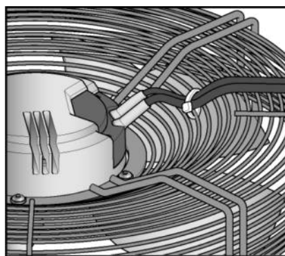
Fig. 1: Fan installed lying flat, cable routed as a water trap.
