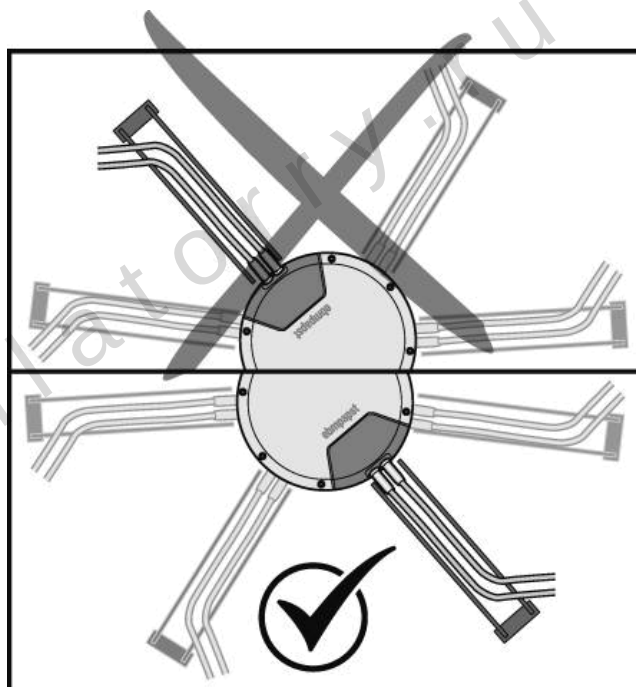
Fig. 2: Cable routing for fans installed in upright position. The cables must always be routed downwards.
