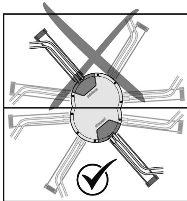
Fig. 2: Cable routing for fans installed upright.
