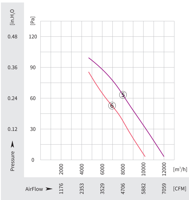
8-Pole
