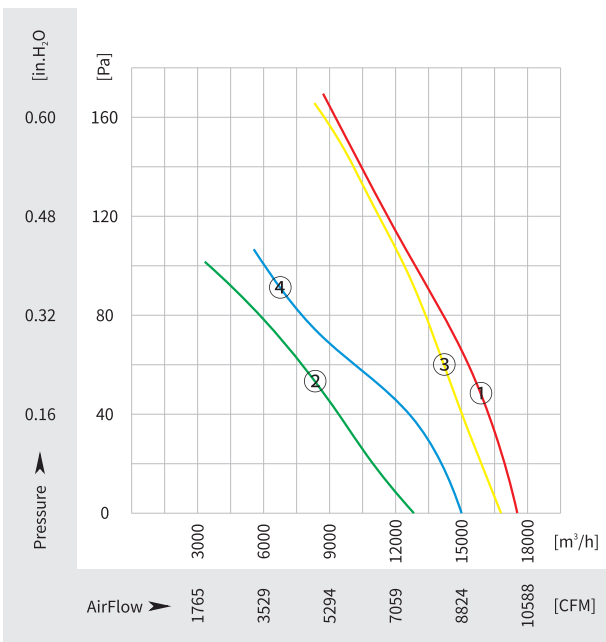
6-Pole
