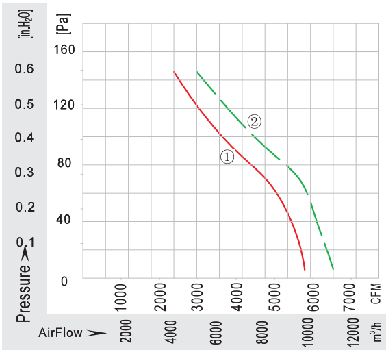
4-Pole
