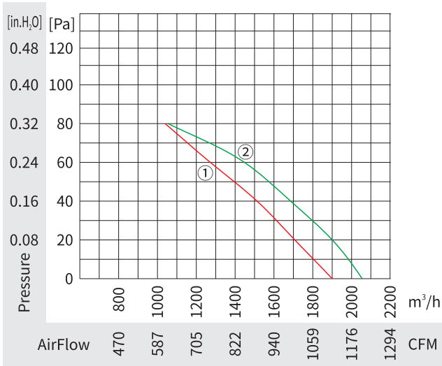
2-Pole
